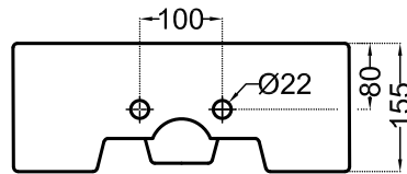
BACK VIEW
