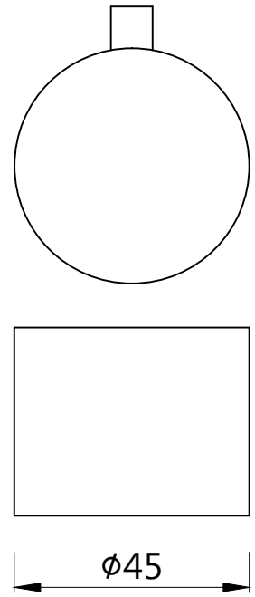
DIVERTER HANDLE
