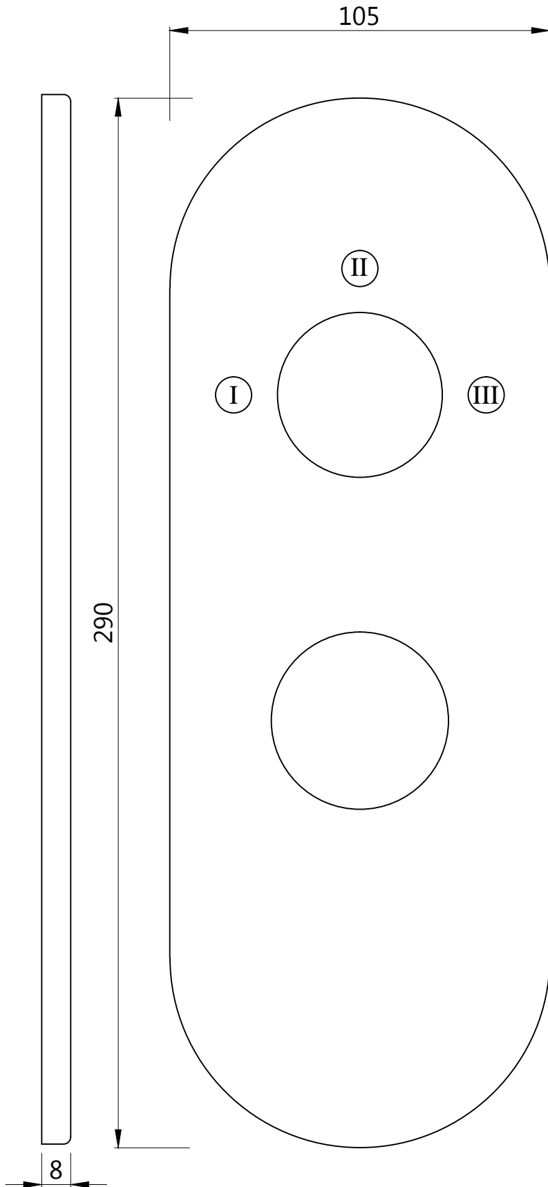
WALL FLANGE
