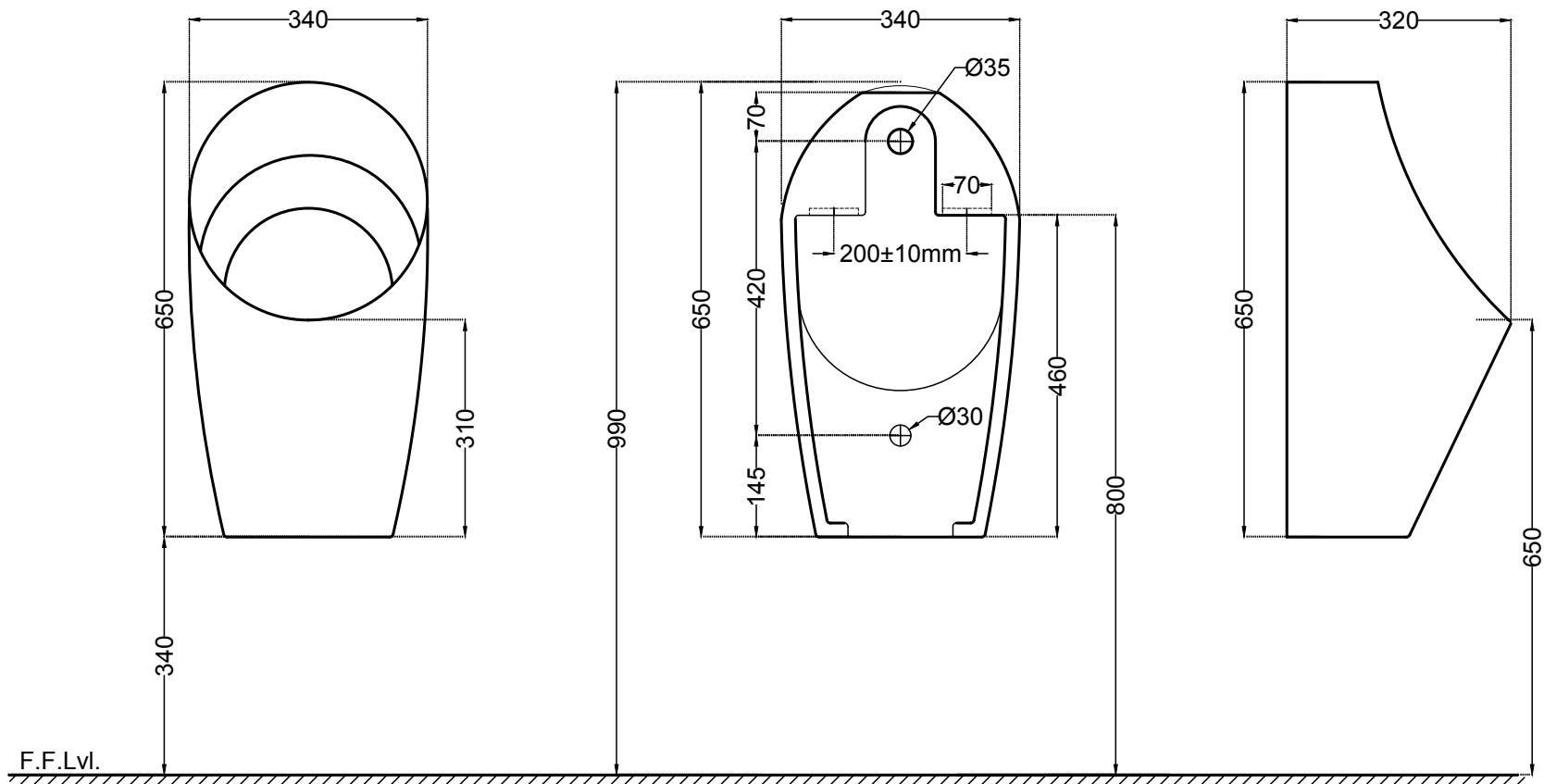
FRONT VIEW
