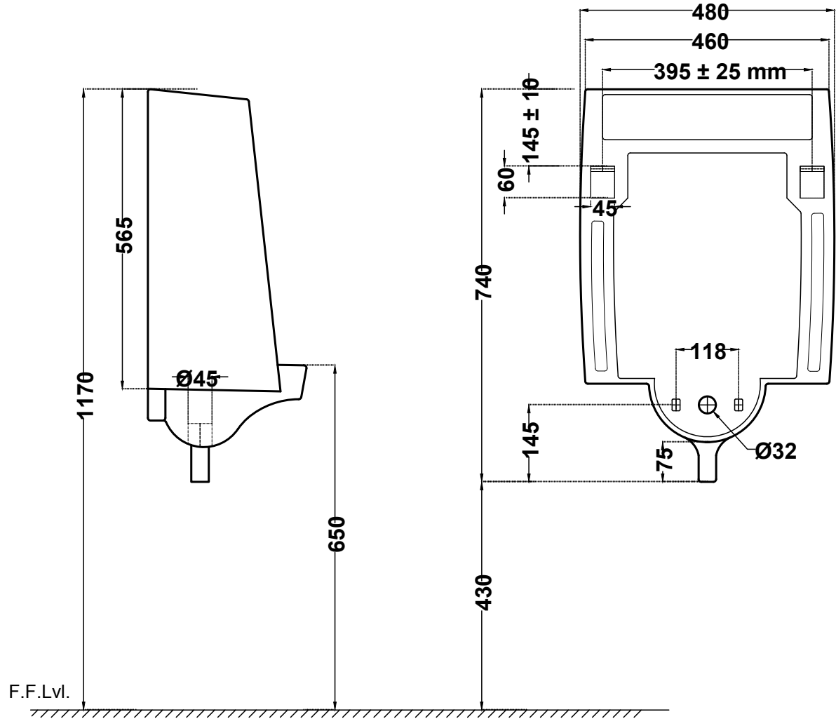
SIDE VIEW
