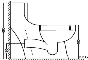
SIDE SECTION
