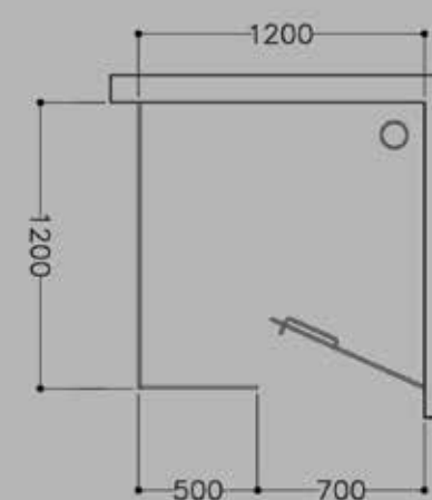
Bathroom Size - 8' x 6' Model Used - 1840 W
