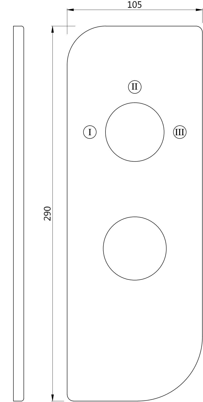
WALL FLANGE
