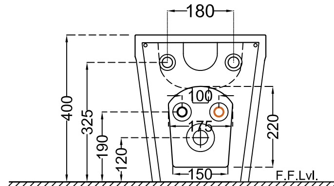
BACK VIEW
