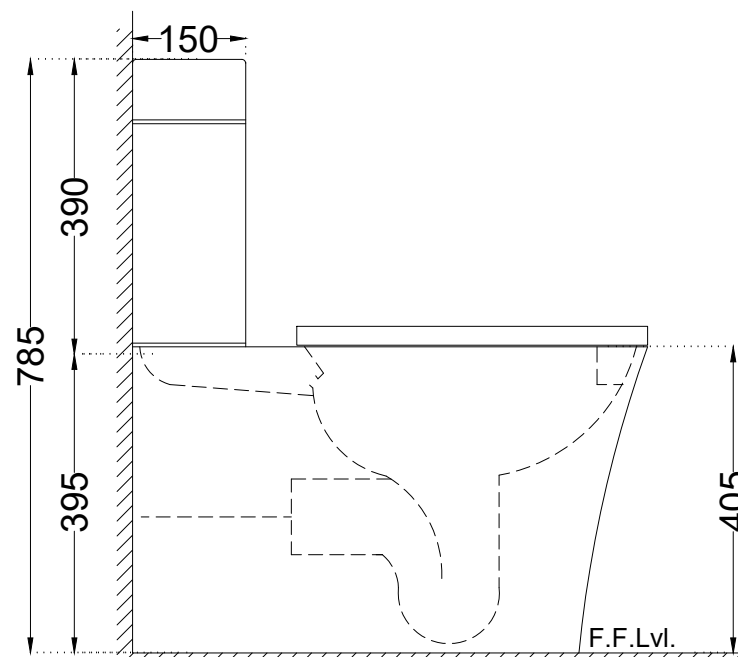
SIDE VIEW
