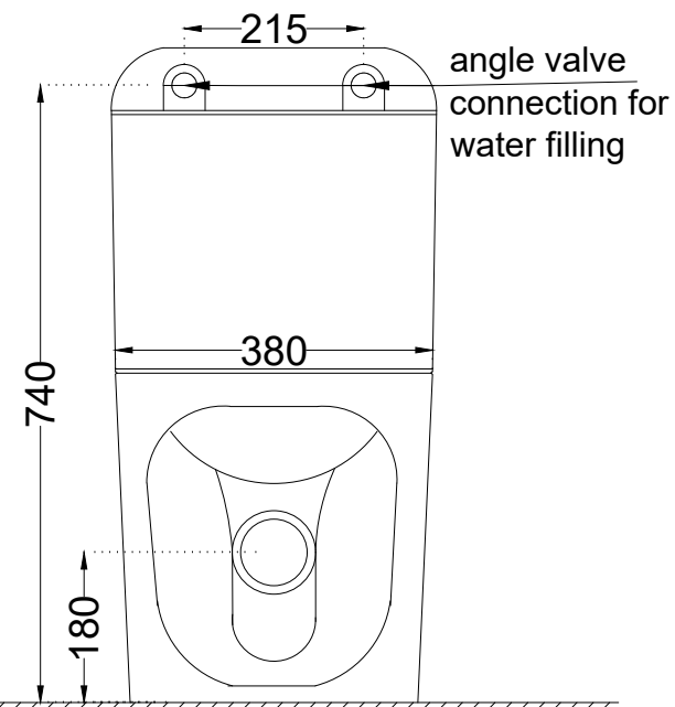
BACK VIEW
