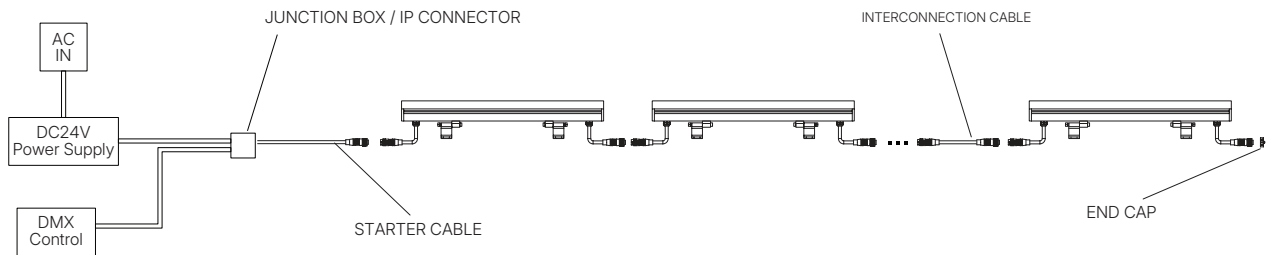
2. Wall Washer Light Wiring diagram of DMX (DC powered version)
