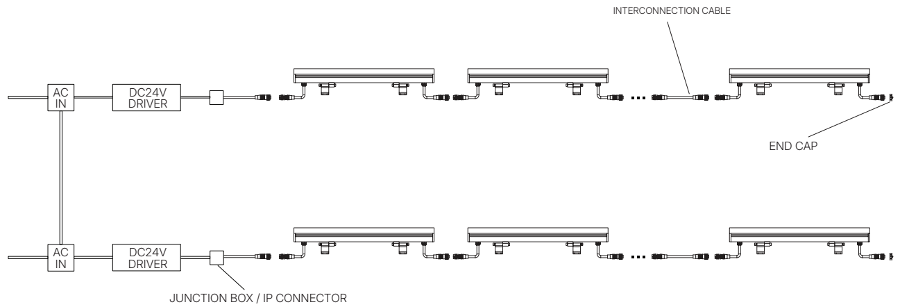
1. Wall Washer Light Wiring diagram of On/Off (DC powered version)
