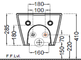
BACK VIEW
