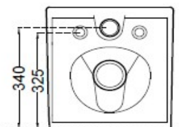
BACK VIEW
