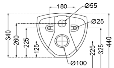
BACK VIEW
