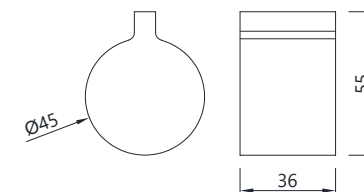
DIVERTER HANDLE
