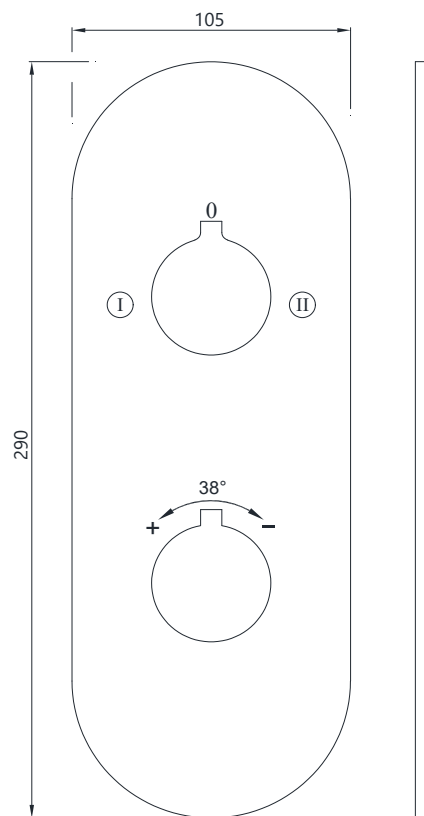
WALL FLANGE
