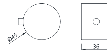
THERMOSTATE HANDLE
